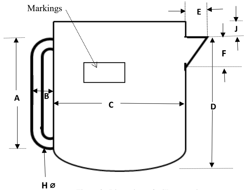
Figure 3 : Dimensions of milk measuring cans
