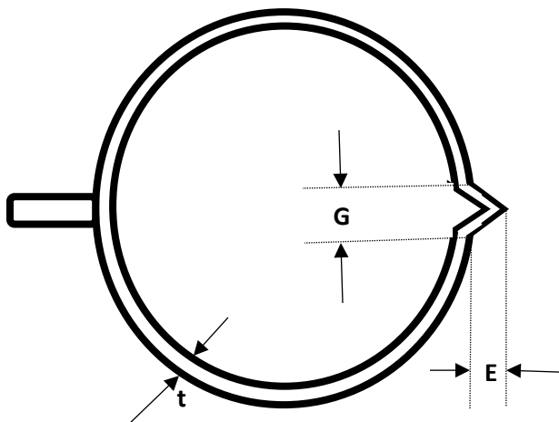
Figure 2 : Dimensions of milk measuring cans
